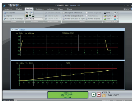
Software
